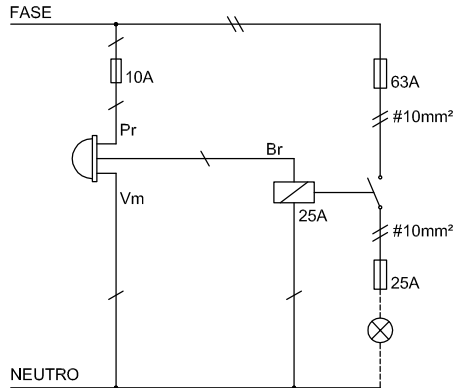
DIAGRAMA UNIFILAR - QC IP 0
