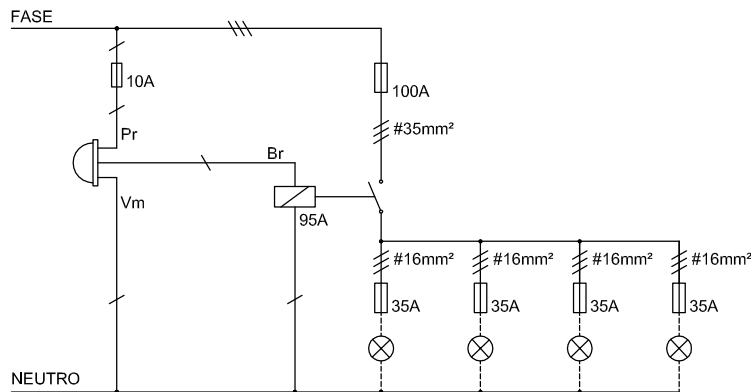
DIAGRAMA UNIFILAR - QC IP 4
