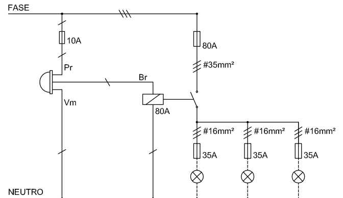
DIAGRAMA UNIFILAR - QC IP 3
