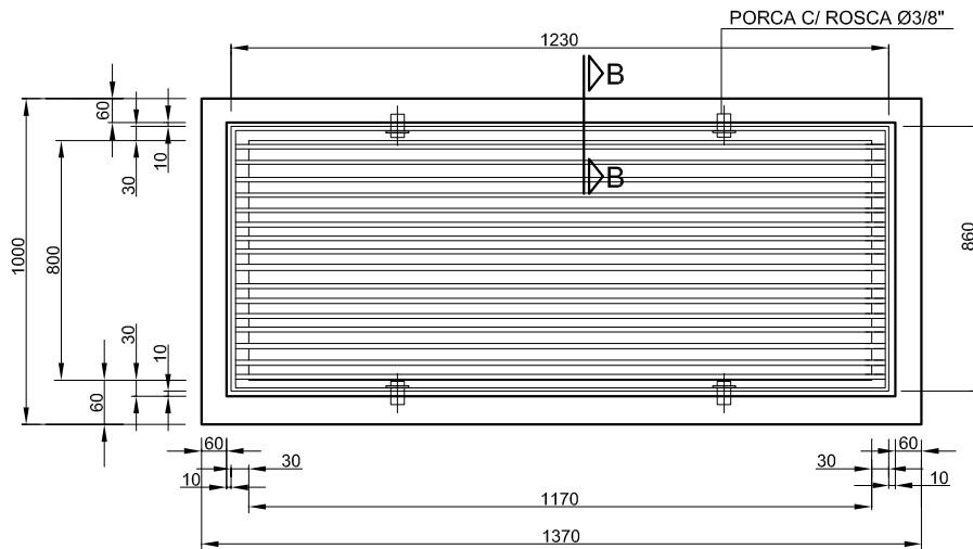
VISTA SUPERIOR COM GRADE
