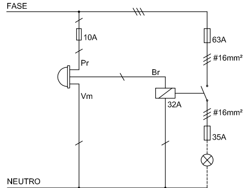
DIAGRAMA UNIFILAR - QC IP 1
