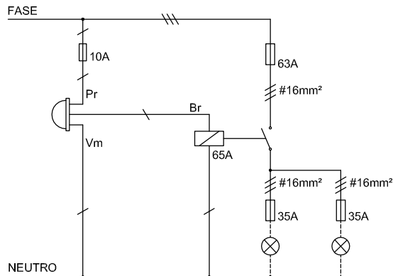
DIAGRAMA UNIFILAR - QC IP 2
